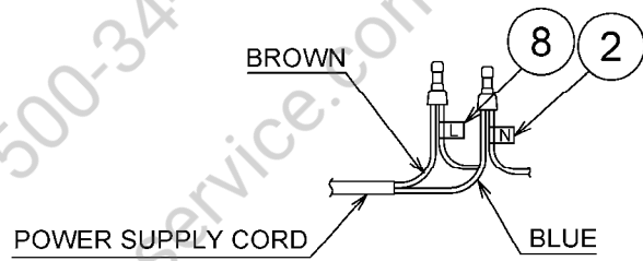
DETAIL LABEL-TERMINAL
